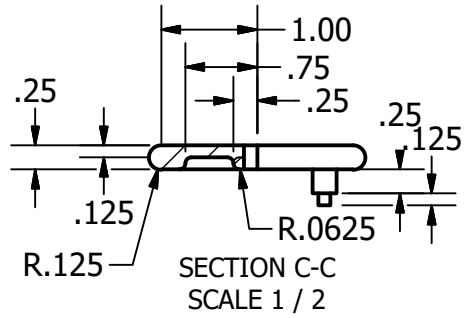
Part #5 Wheel
